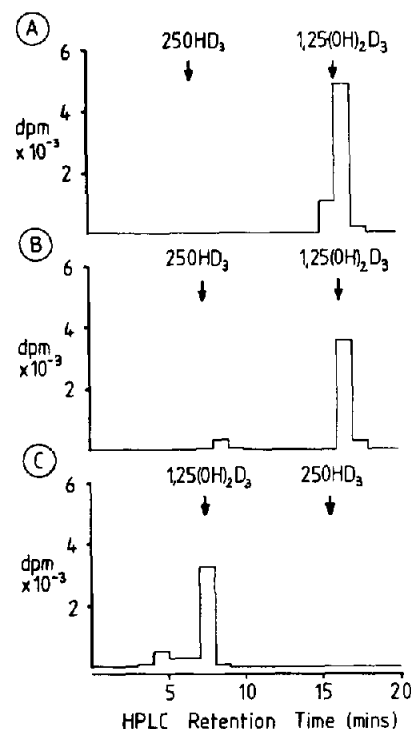
Fig.2. Rechromatography of pooled [ ^3\text{H} ] 1,25(\text{OH})_2\text{D}_3 produced by peritoneal M \phi , following initial chromatography on HPLC system (A), from patients with a history of peritonitis on 3 HPLC systems. (A) Zorbax-SIL column eluted at 1.5 ml/min with n -hexane, propan-2-ol, methanol (110:6:4), (B) Zorbax-SIL column eluted at 1 ml/min with 2.5% methanol in dichloromethane, (C) Zorbax-ODS reverse-phase column eluted at 2 ml/min with 15% water in methanol. Bars represent the amount of tritiated material in 1-ml fractions and the arrows indicate retention times of standard 25OHD _3 and 1\alpha,25(\text{OH})_2\text{D}_3 determined by UV absorbance (265 nm).
